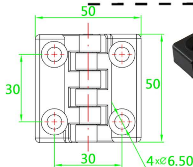
Small hinge
