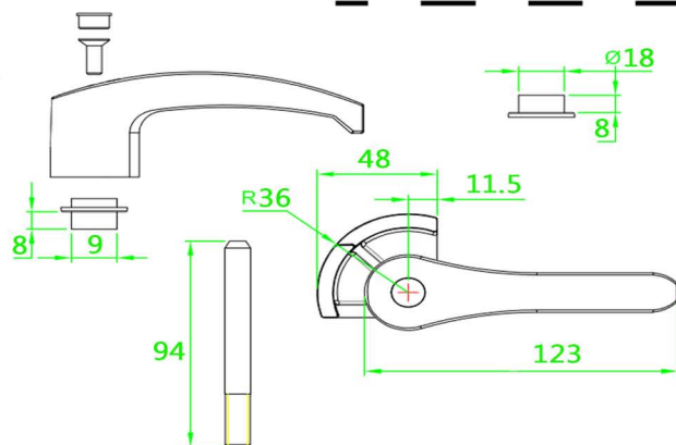
Rotary Handle 1 and 2 inch Plastic
