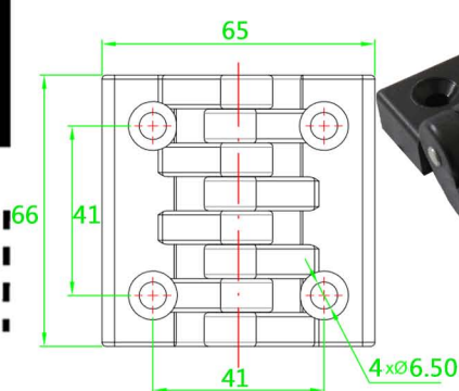
Large hinge
