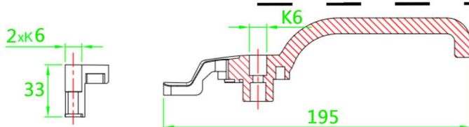
Rotary Handle 1 and 2 inch Plastic
