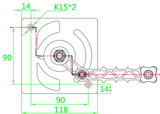
Damper handle Plastic
