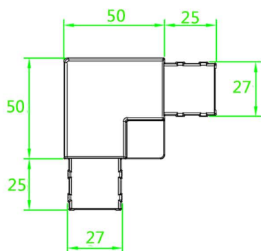
Corner 3 cm Aluminum
