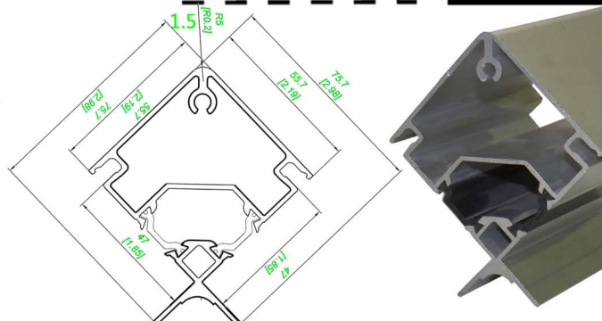
Thermal Break Corner Post 5cm
