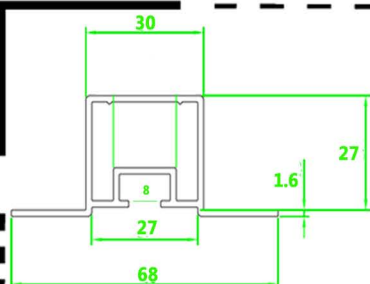
Corner 3 cm Aluminum
