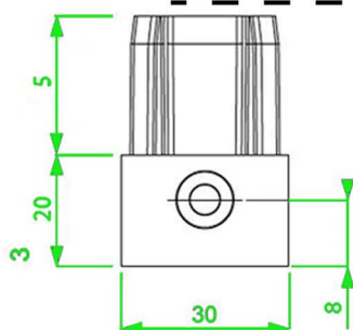
Top Hat Connection 3cm Plastic
