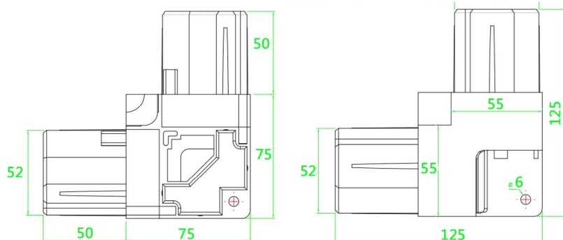
Thermal Break Corner 5 cm Plastic
