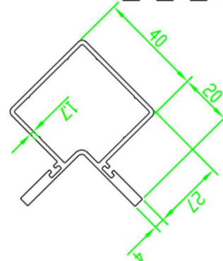
Corner Post 4 cm
