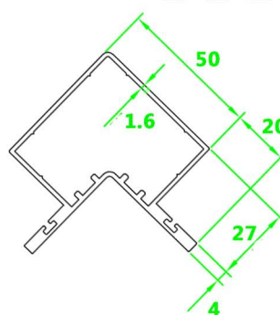
Corner Post 5 cm
