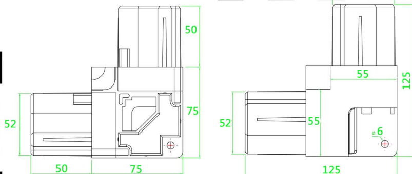
Hygienic Corner 5 cm Plastic
