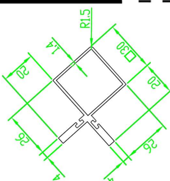
Corner Post 3cm
