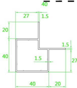
Corner Post 4 cm
