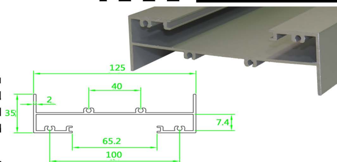
Damper Profile
