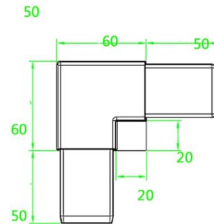
Corner 4 cm Aluminum
