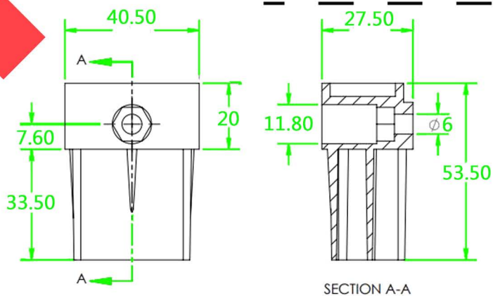
Top Hat Connection 4cm Plastic
