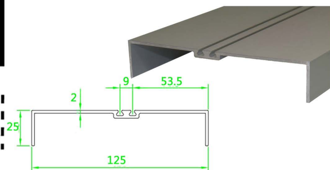
Damper profile
