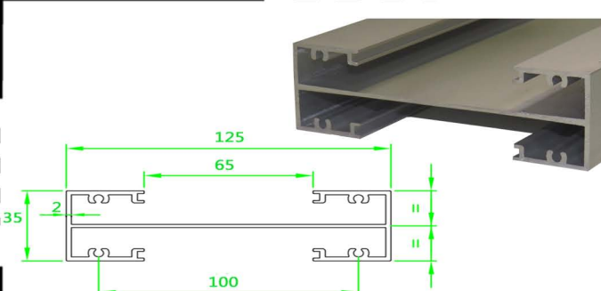
Damper Profile
