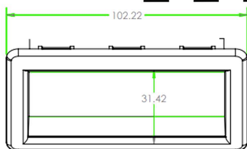
Handle Plastic
