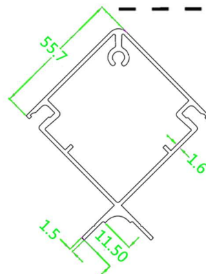
Hygienic Corner Post 5 cm
