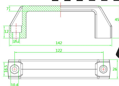
Handle 4001
