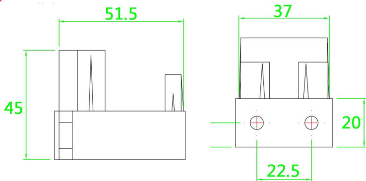
Thermal Break Top Hat Connection 5cm Plastic
