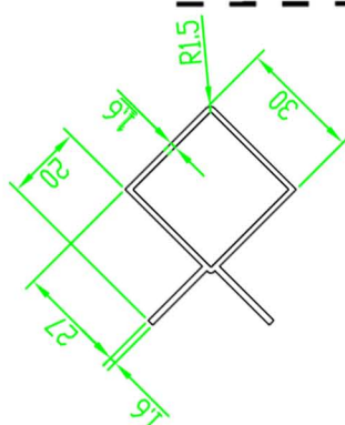
Corner Post 3cm
