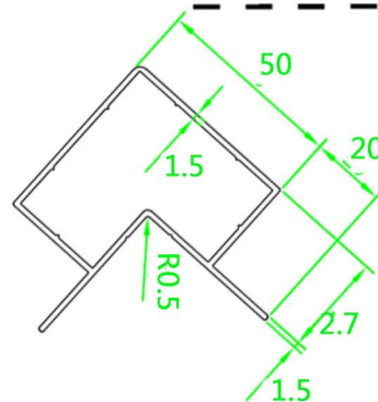
Corner Post 5cm
