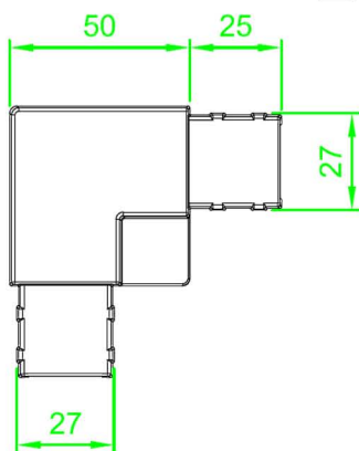
Corner 3 Plastic
