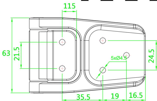
Plastic hinge
