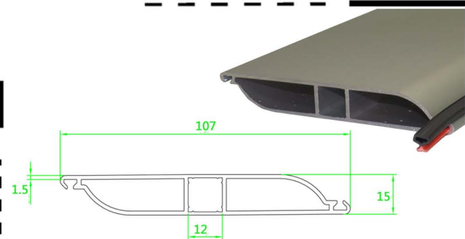
Damper profile
