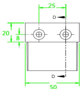
Top Hat connection 5 cm Plastic
