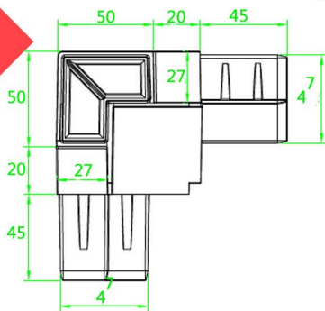
Corner 5 cm Aluminum & Plastic Weight: 739.227 gr
