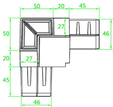
Corner 5 cm Aluminum & Plastic
