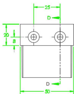
Top Hat Connection 5cm Plastic Weight: 30 gr
