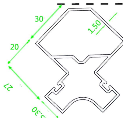
Hygienic Corner Post 4cm
