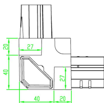
Hygienic Corner 4cm Material: Plastic
