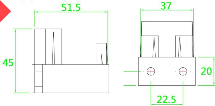
Hygienic Top Hat Connection Plastic
